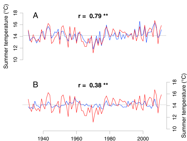
Figure 3. Comparison between reconstructed (blue) and observed (red) summer temperature from Bariloche station over the calibration period 1931–2011 for the (A) \delta^{13}C_{cor} -based and (B) BAI res -based regression models. The standard deviation of the summer temperature series is 1.12 for the observation and 0.89 (0.39) for the reconstruction based on \delta^{13}C_{cor} (BAI res ) over the 1931–2011 period. The ** indicates that the correlation is significant at 99% confidence level.
