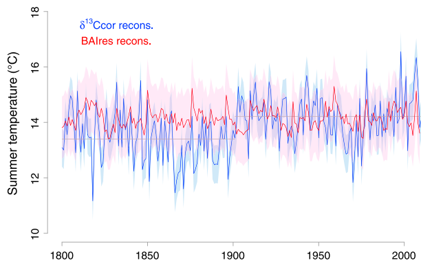
Figure 4. Summer temperature reconstruction variations based on \delta^{13}\text{C}_{\text{cor}} (blue) and averaged \text{BAI}_{\text{res}} (red) over the period 1800–2011. The shaded blue (red) represents the confidence intervals ( \pm\text{RMSE} = 0.69^\circ\text{C} or 1.15^\circ\text{C} , respectively). The changes in mean temperature levels detected with the Pettitt’s test for the reconstruction based on \delta^{13}\text{C}_{\text{cor}} are shown in gray (mean of 13.4^\circ\text{C} before 1903 and 14.2^\circ\text{C} after 1903).
